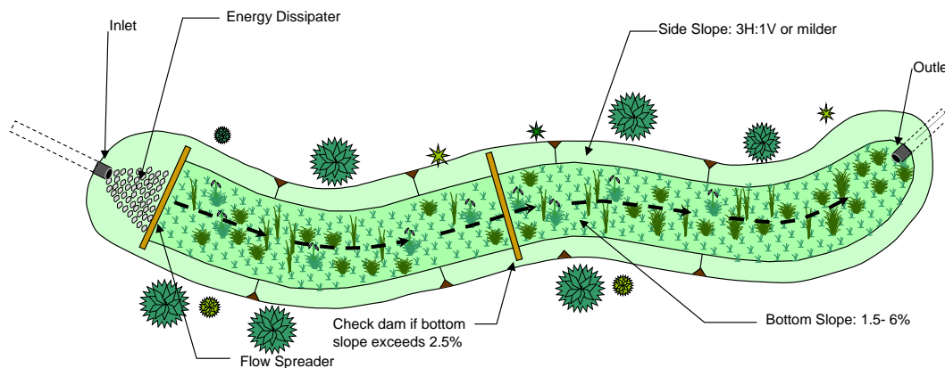
Figure 5-10. Schematic of a Vegetated Swale
