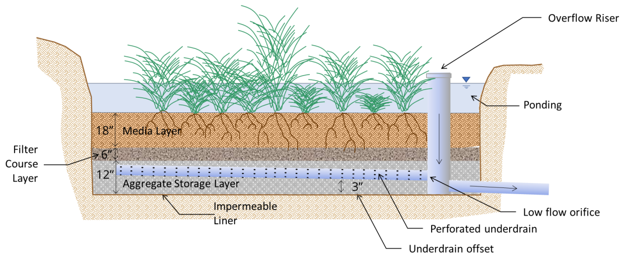
Biofiltration BMP Example Illustration
