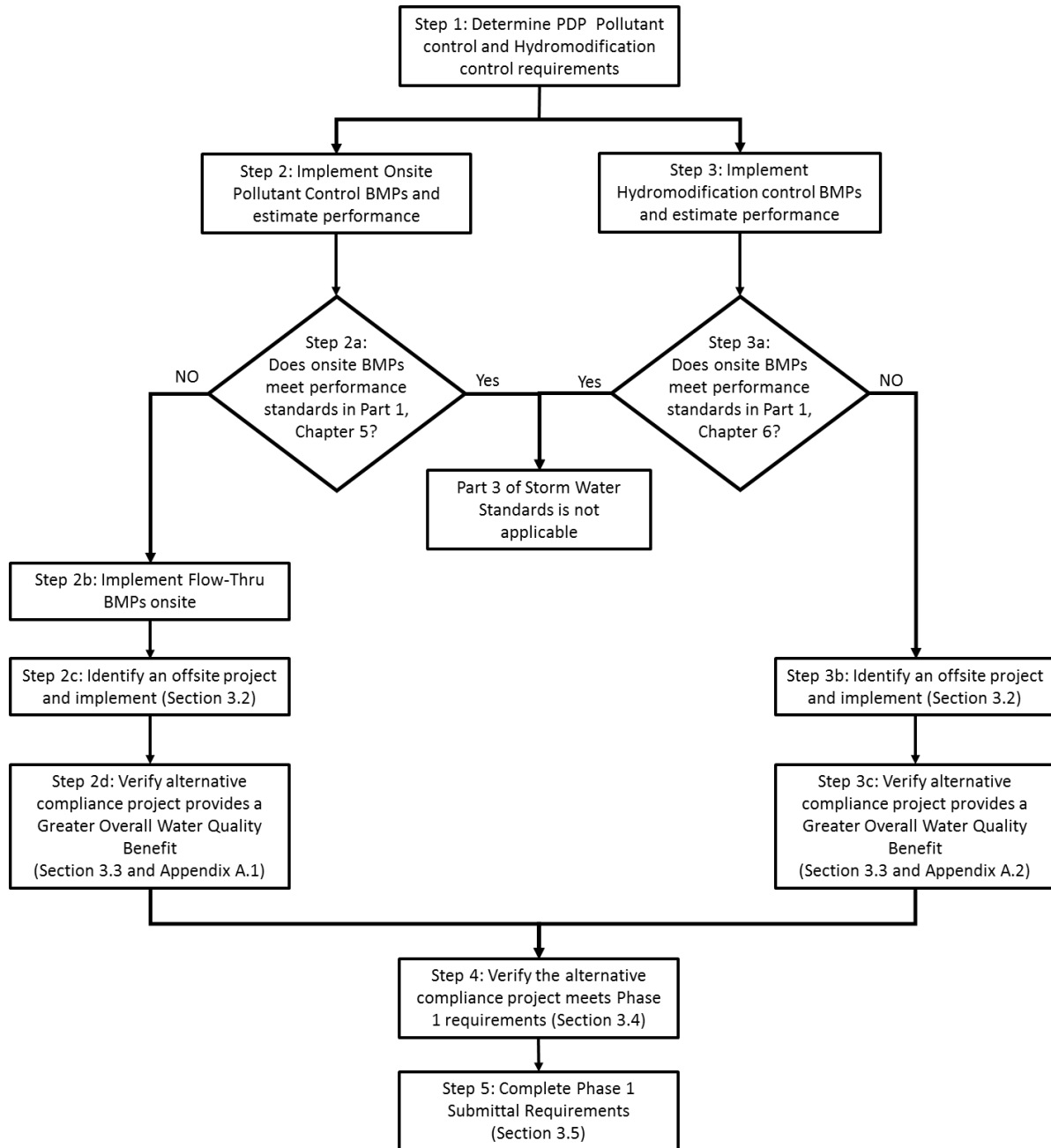
Figure 3-1. Phase 1 Alternative Compliance Program Process
